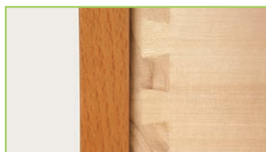
Hardwood drawer box construction with double drawer fronts and English dovetail joinery for extra strength.
