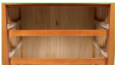
Solid beech posts joined with mortise and tenon parting rails for maximum structural support.
